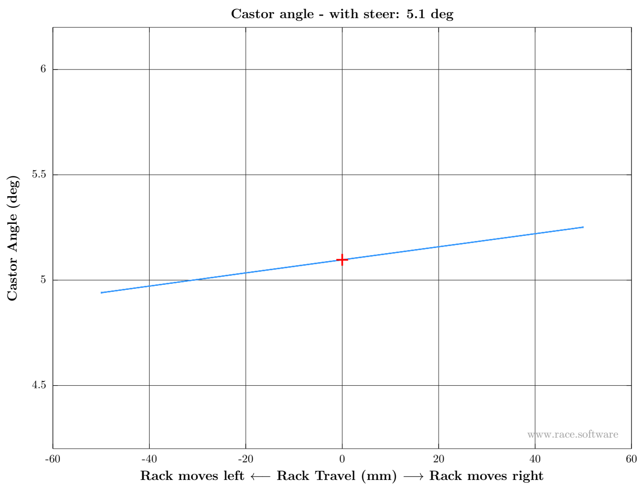
Figure 18: Steering test: Caster angle - with steer
