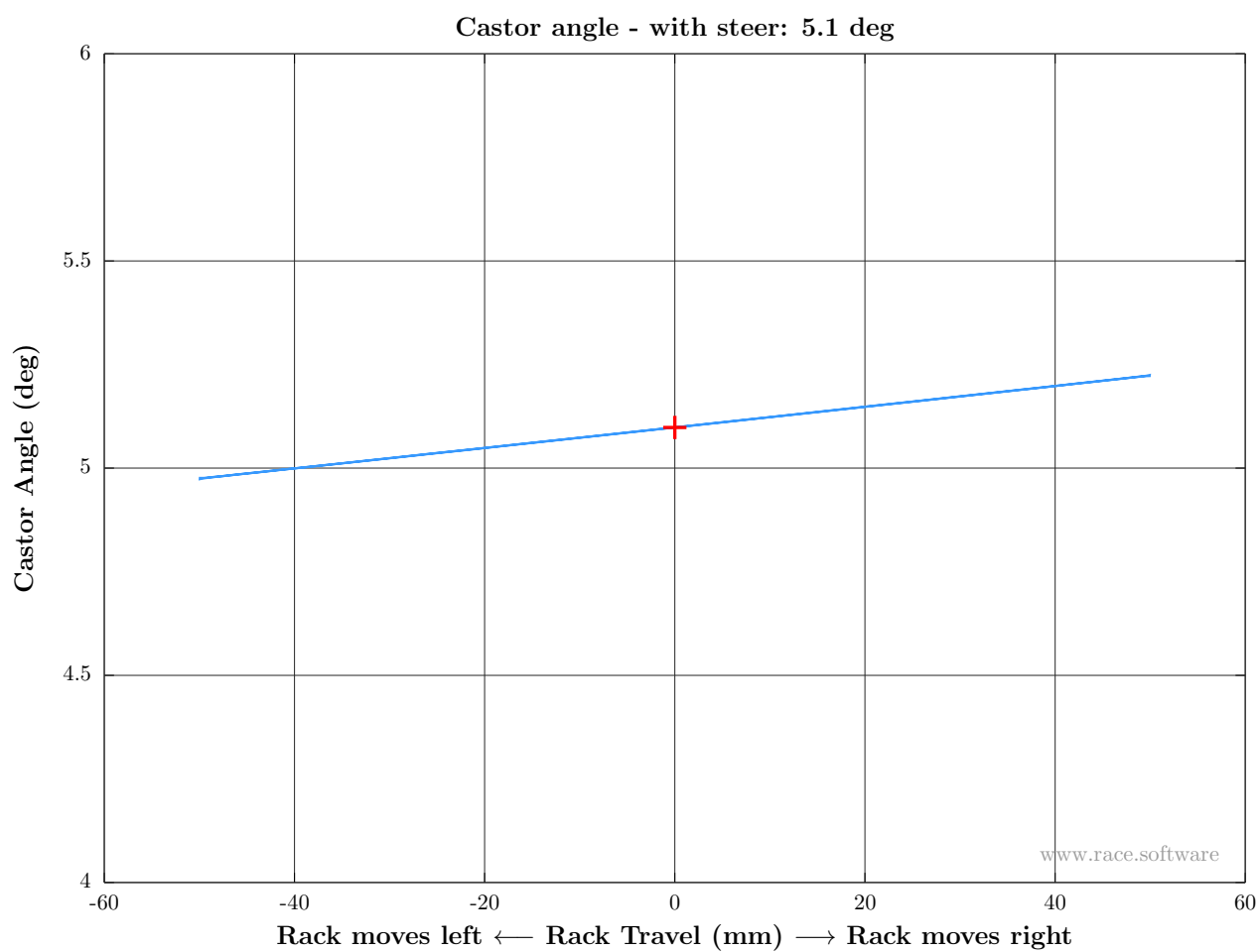
Figure 38: Steering test: Caster angle - with steer
